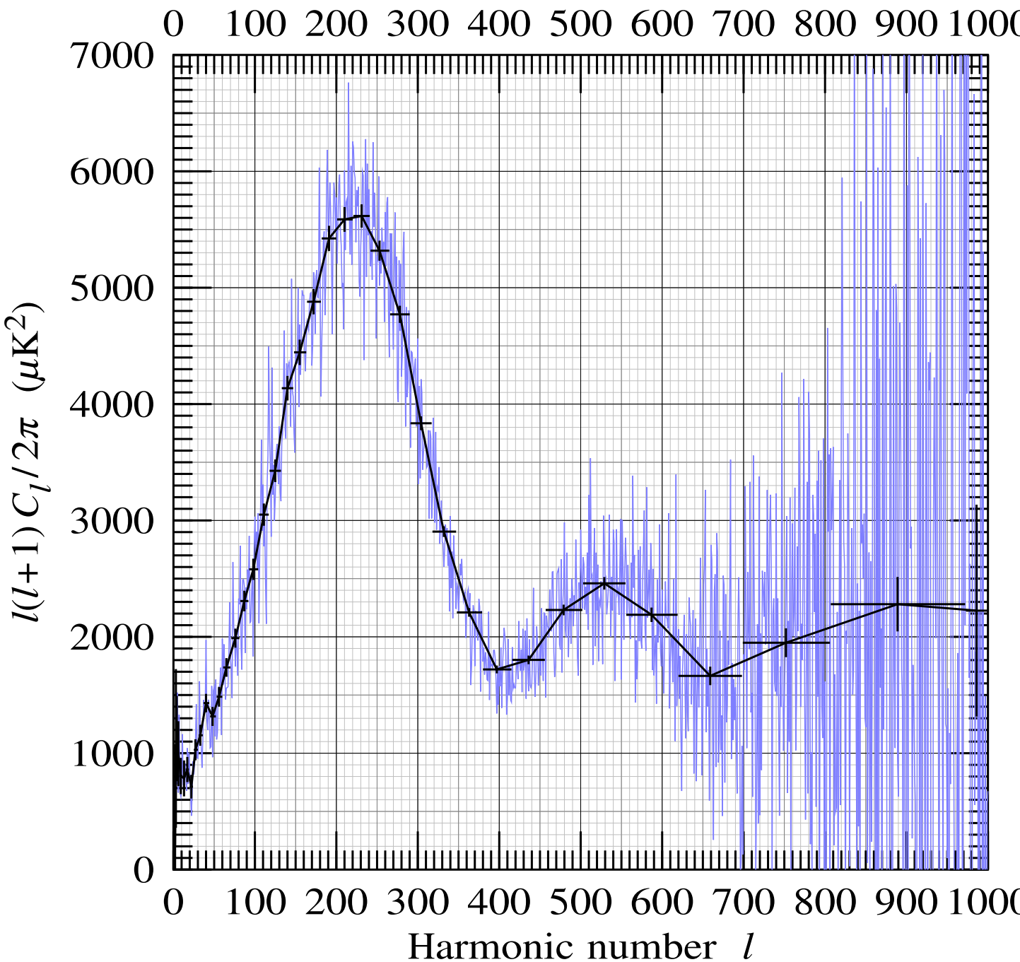
WMAP 3-year power spectrum (2006)
